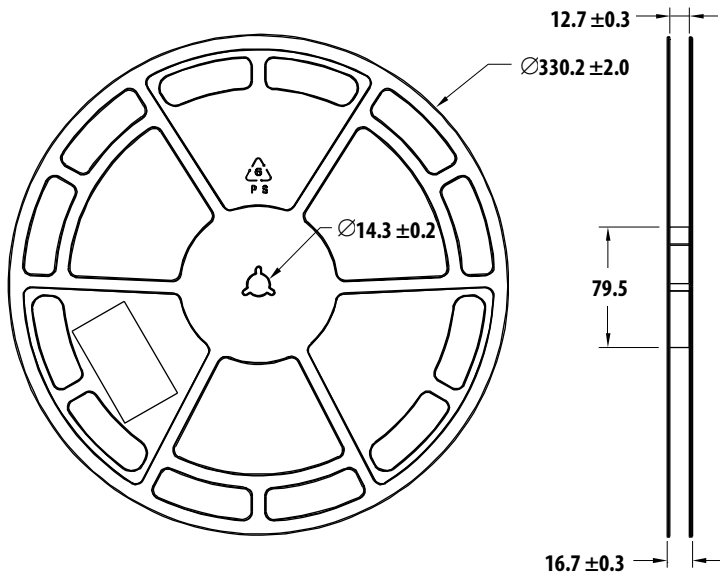
Figure 14: Reel Dimensions
